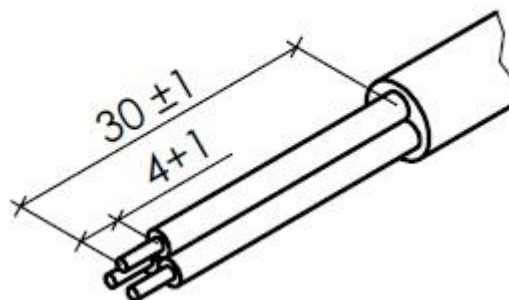
Stripping of solid conductors and stripping of the outer sheath
